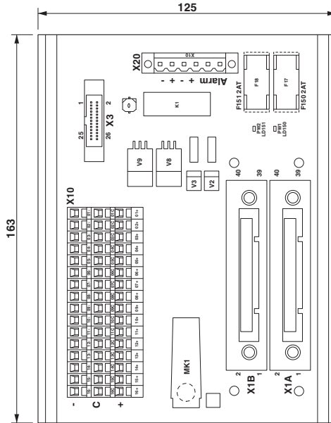
Dimensional drawing
