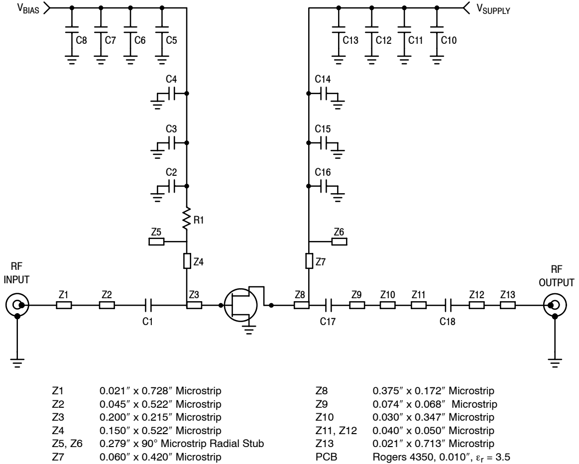
Figure 1. MRFG35020A Test Circuit Schematic
